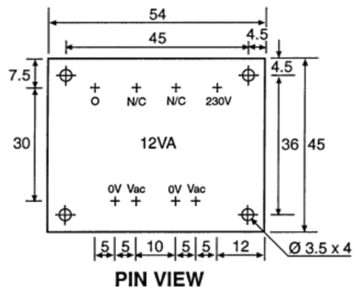
PIN VIEW
